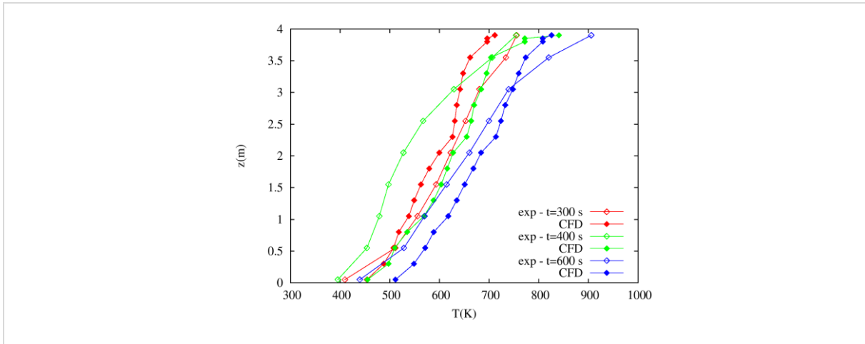
Figure 16: Comparison between the experimental and numerical gas temperature in the fire room at three times for the test PR2_VSP_3.
