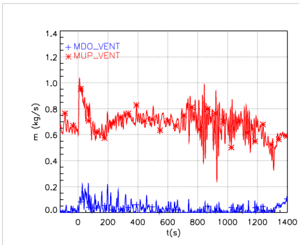
Figure 8: Time variation of the upward (UP) and downward (DO) air mass flow rate at the vent
