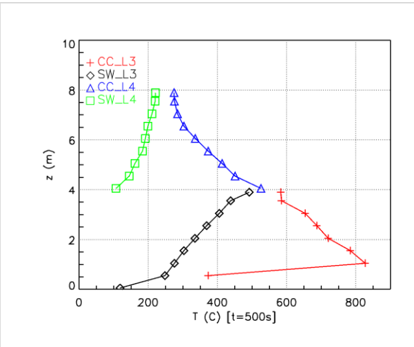
Figure 7: Vertical temperature profiles at the axis of the vent (CC) and on the SW axis in the fire room L3 ( z=[0;4] m) and in the upper room L4 ( z=[4;8] m) at t=500 s.
