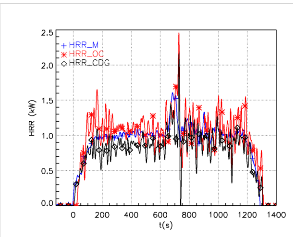
Figure 9: Time variation of the fire Heat release rate computed from mechanical (M), CDG and OC methods
