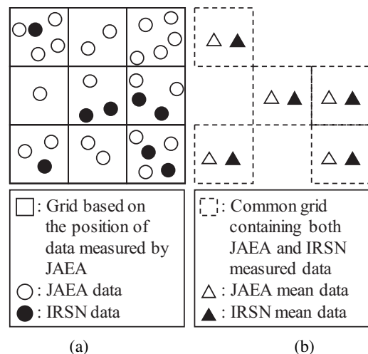
Fig. 13. Establishment of the grid used to calculate the average air dose rate. (a) Creation of the grid based on the location information of JAEA's measurement data and (b) extraction of the common grid of the measured data of both JAEA and IRSN.
