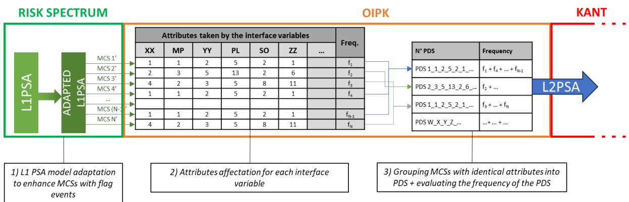
Figure 2. Main Steps of L1/L2 PSA Interface
